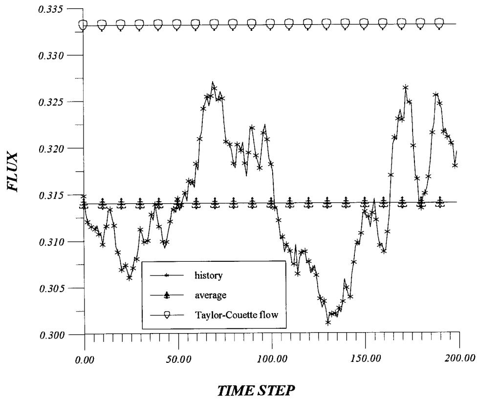
Figure 4: Flux of the flow.
