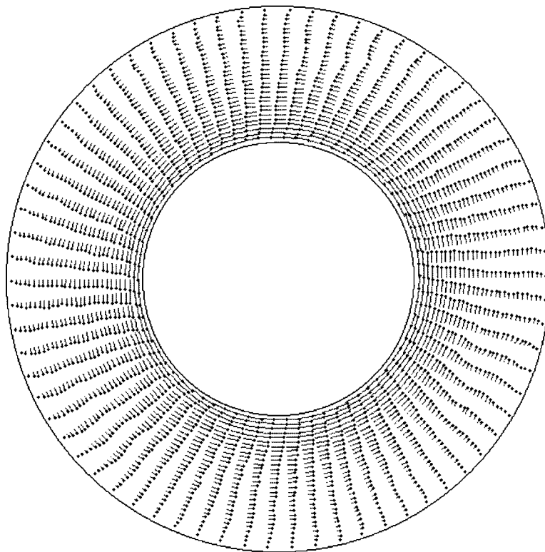
Figure 3: Time-averaged velocity field.
