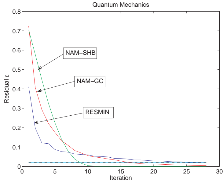
FIGURE 4. First results on a small Quantum mechanics test case
