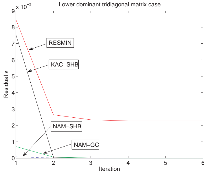
FIGURE 3. Convergence Speed of some tested Algorithms in the tri-diagonal case
