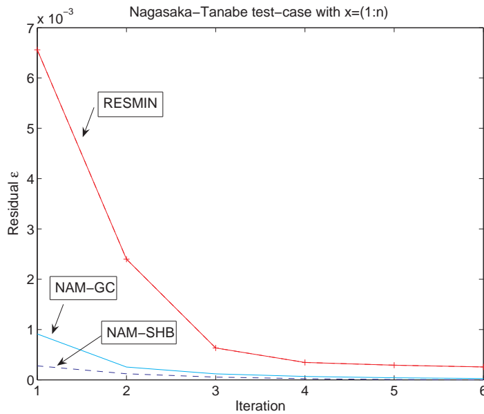
FIGURE 1. Convergence Speed of some tested Algorithms in the Nagasaka case
