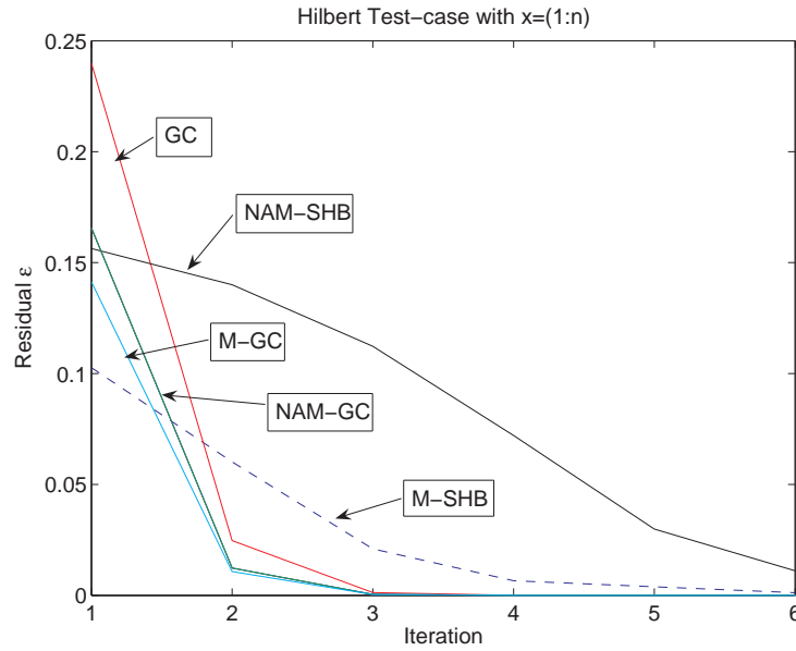
FIGURE 2. Convergence Speed of some tested Algorithms in the Hilbert case
