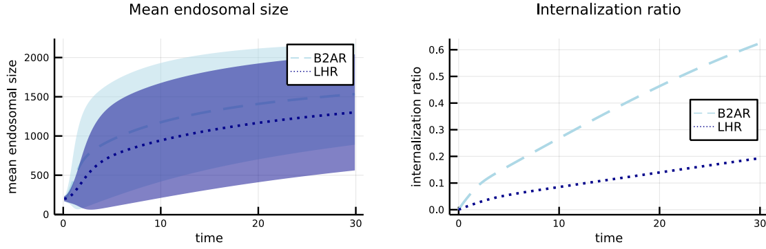
FIGURE 7. Time evolution of the endosomal size (left panel) and internalization ratio (right panel). We numerically simulate the 2D model given by Eqs. (M2a)-(M2b) with parameters given by. (35)-(36)-(37) (LHR and B2AR affect only the internalization rate). On the left panel, the dashed blue (resp. dotted purple) line represents the mean endosomal size for B2AR (resp. LHR), that corresponds to \|f\|_{1,0}(t)/\|f\|_{0,0}(t) , and the shaded light area represents its standard deviation. On the right panel, the dashed blue (resp. dotted purple) line represents the internalization ratio for B2AR (resp. LHR), that corresponds to \frac{\|f\|_{0,1}(t)}{M_0} .
