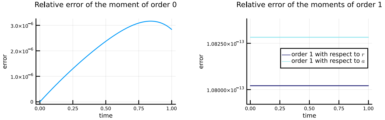
FIGURE 2. Relative error of the moments of order 0 (left panel) and 1 (right panel) between moments computed from our pure coagulation numerical scheme (21) and from the analytical solution of the ODE system Eq. (23), in the case of a constant kernel (26) with the same parameters as in the left panel of Figure 1.
