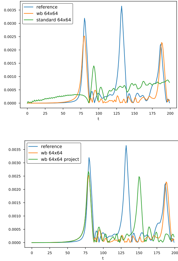
FIGURE 8. Time history of the quantity (23). Left: comparison of the standard scheme and the well-balanced scheme on a 64 \times 64 mesh. Right: comparison of the well-balanced scheme with and without projection on a 64 \times 64 mesh.
