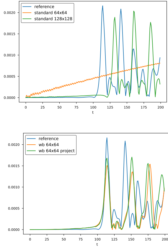
FIGURE 6. Time history of the quantity (23) for b = 1.12 + \sqrt{2} . Left: standard scheme on a 64 \times 64 and 128 \times 128 meshes. Right: well-balanced scheme on a 64 \times 64 with and without a projection at t = 115 (until t = 115 the two schemes overlapped). The well-balanced scheme gives better results even on coarse meshes.
