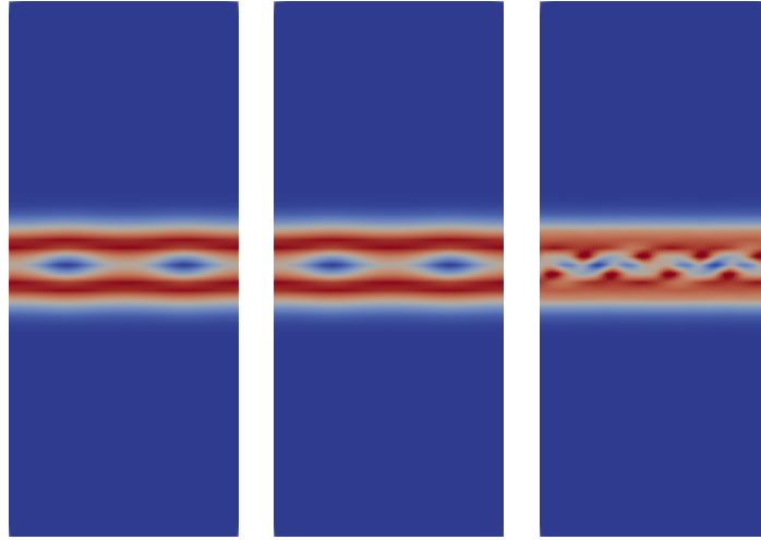
FIGURE 3. Phase space representation of the function f^+ for the first stable numerical test with no perturbation. From left to right: initial condition, well-balanced scheme at T = 200 , standard scheme at T = 200 .
