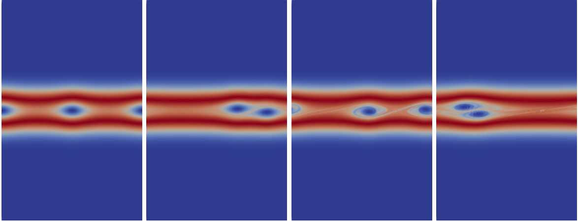
FIGURE 7. Phase space representation of the function f^+ at different times of the simulation for the test case 4.4 where b = 1 + \sqrt{2} . From left to right: t = 0 , t = 75 , t = 100 and t = 130 . The holes interact but do not merge.
