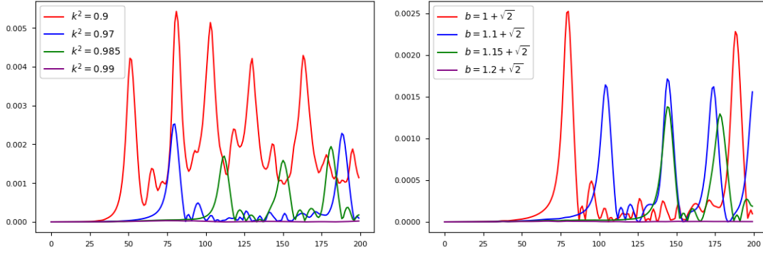
FIGURE 2. Left figure: time evolution of (23) for different values of k (the other parameters are a = -1, \lambda = b = 1, m = k^2, x_0 = 0 ) ; right figure: time evolution of (23) for different values of b (the other parameters are a = -1, \lambda = 1, m = k^2 = 0.97, x_0 = 0 ). For both figures, L = 4K(k) .
