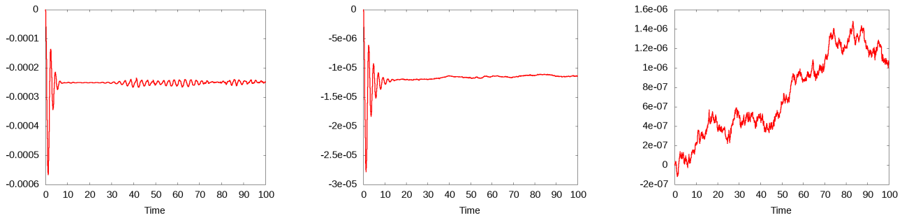
FIGURE 1. Time evolution of the relative error on the total energy for three values of the perturbations. At the left \alpha = 0.5 , in the middle \alpha = 0.1 , and at the right \alpha = 0.005 .
