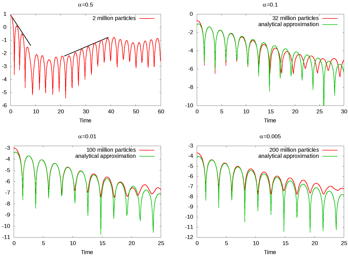
FIGURE 2. Time evolution of the log of the electric field energy for four values of \alpha . The time step is 0.1 and the grid has 128 \times 2 cells. When \alpha = 0.5 , the slopes for the initial damping and for the growth between t = 20 and t = 40 are -0.2920 and 0.0815 respectively (see [5]).
