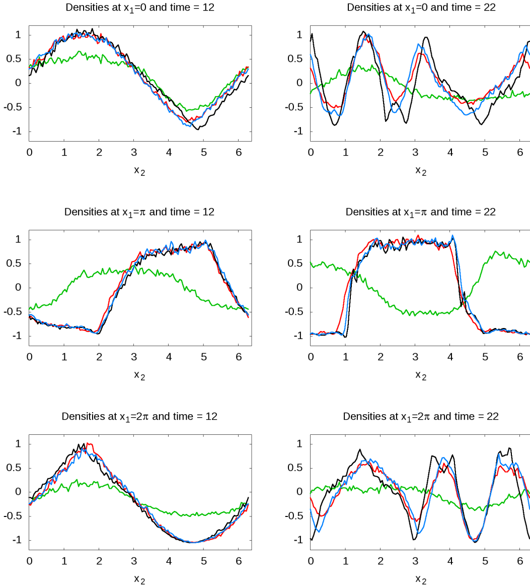
FIGURE 8. The Kelvin-Helmholtz instability with 10 million particles and \Delta t = 0.01 : Cuts in different x_1 directions of the densities of the guiding center model (in black), the Vlasov-Poisson model with \varepsilon = 0.05 (in blue), with \varepsilon = 0.1 (in red), and with \varepsilon = 0.5 (in green). The final times are 12 (at left) and 22 (at right).
