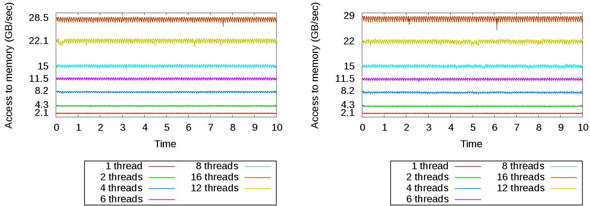
FIGURE 5. History of the instantaneous memory bandwidth in GB per second (as measured during the particle push loop only) for the 2 million (left) and 20 million (right) particles runs, with multithreading.
